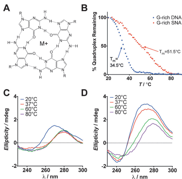
Figure 1. A) G-quartet structure stabilized by M^+ ( Na^+ , K^+ , etc.) B) CD spectroscopy was used to measure the melting temperature ( T_m ) of G-quadruplexes formed on the SNA and with linear G-rich DNA. The full CD spectra for C) G-rich DNA and D) G-rich SNAs are shown at increasing temperatures, demonstrating the enhanced thermal stability of G-quadruplexes formed on the SNA scaffold.
